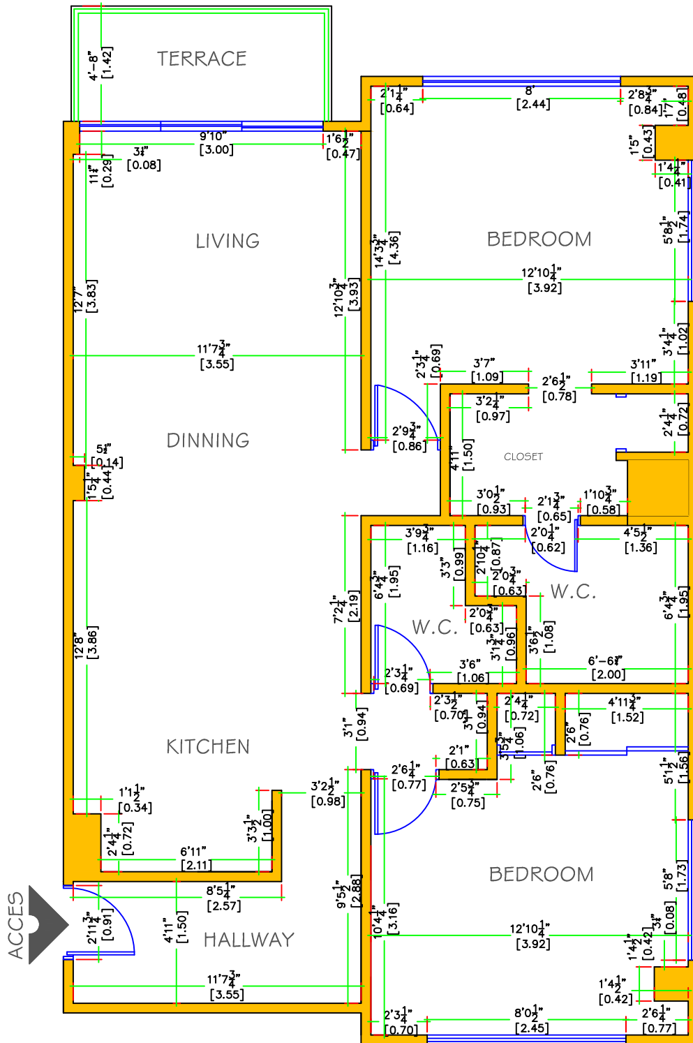
FLOOR PLAN
