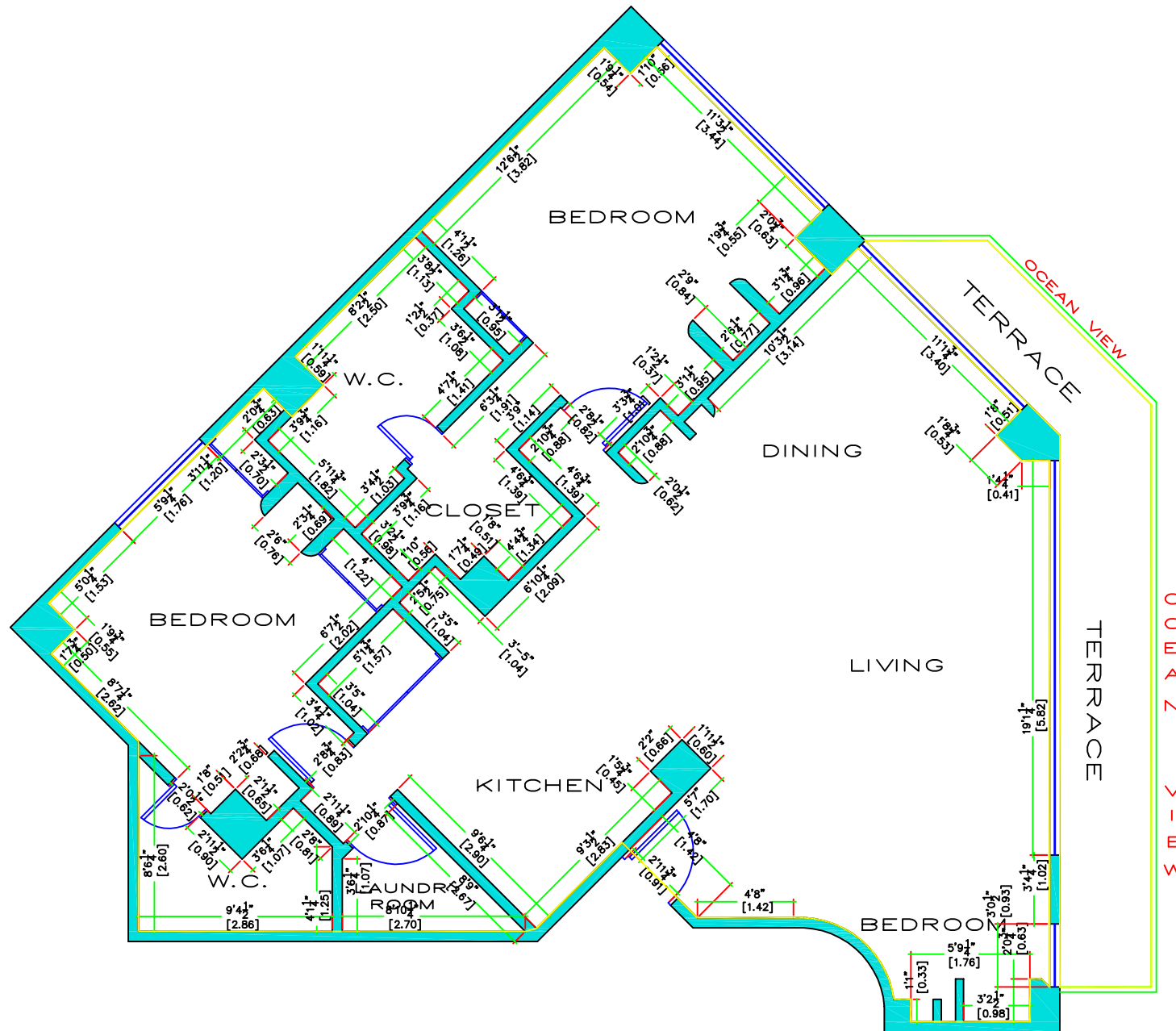
FLOOR PLAN
