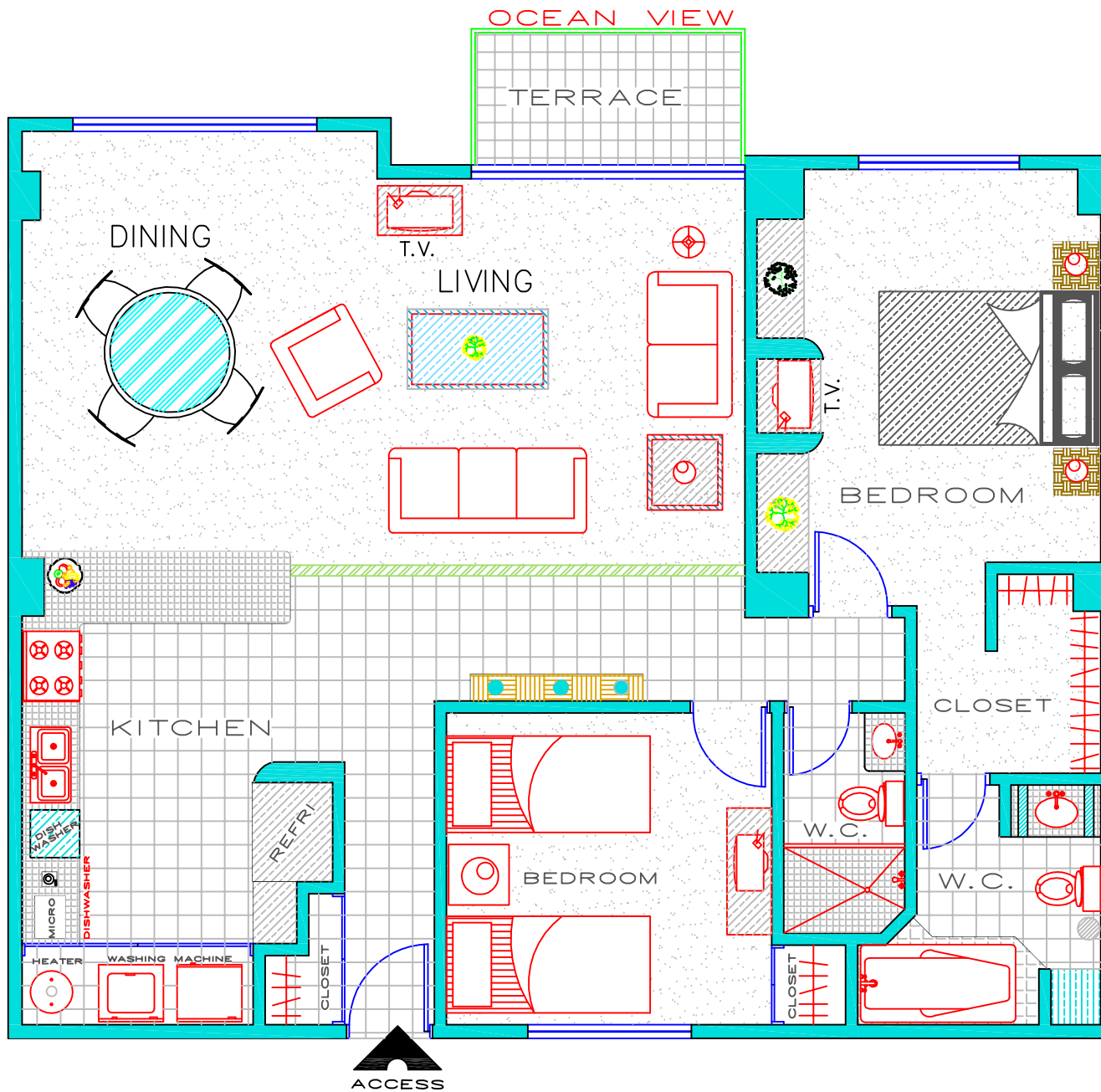
FLOOR PLAN
