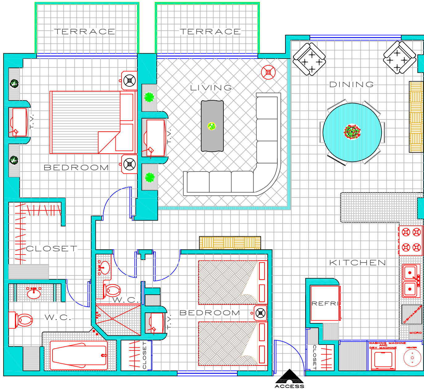
FLOOR PLAN
