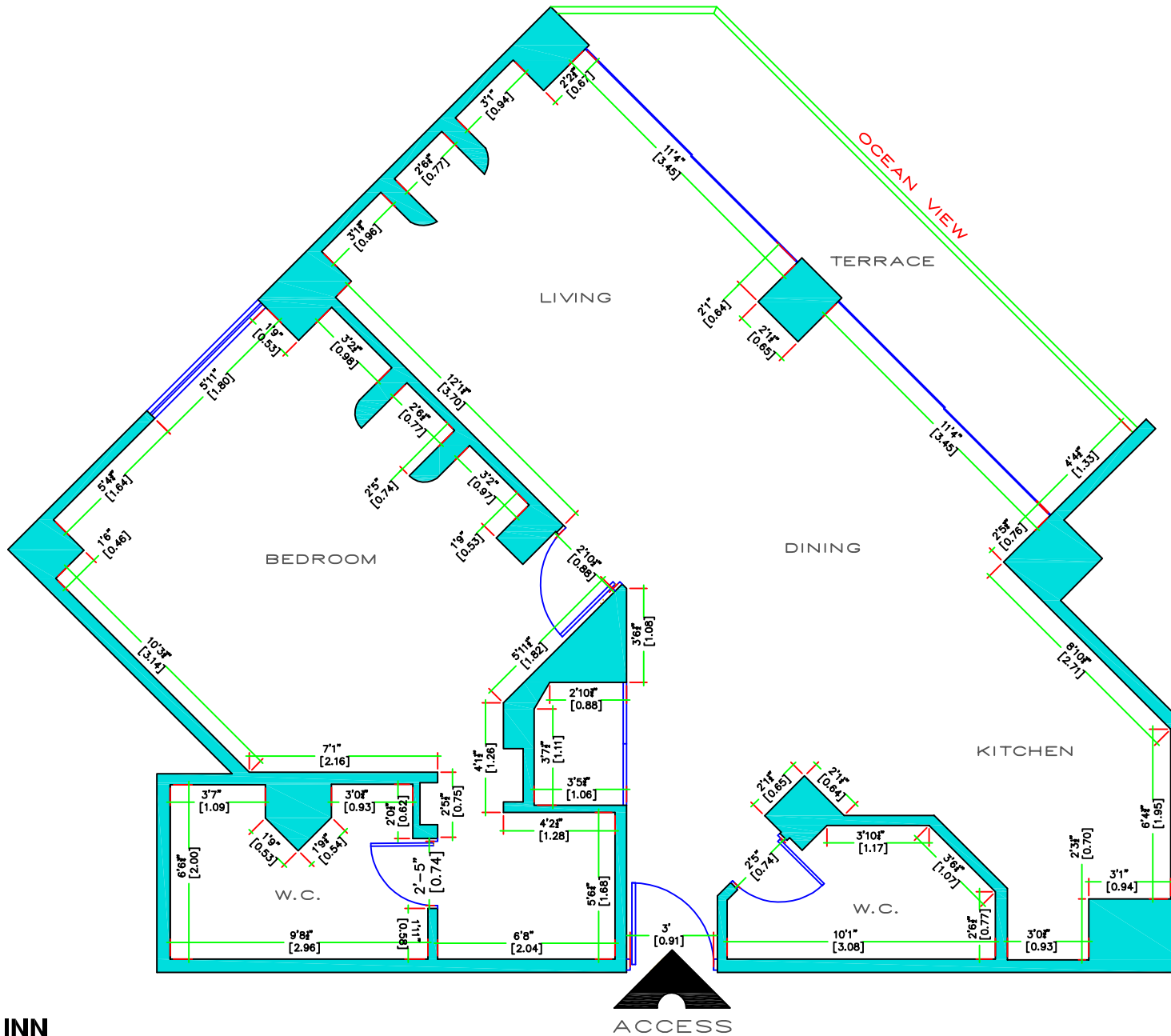
FLOOR PLAN
