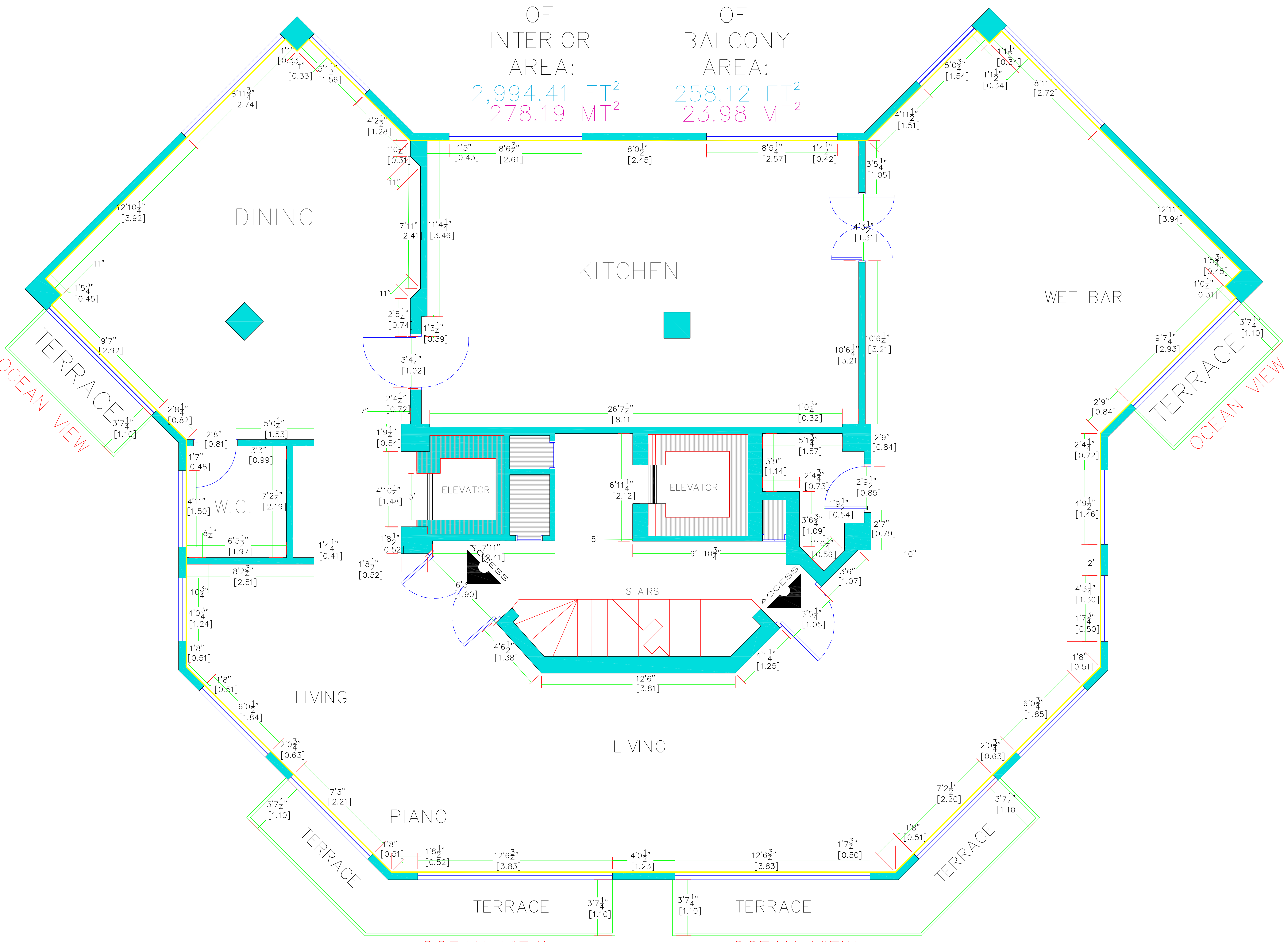
OCEAN VIEW OCEAN VIEW ARCHITECTURAL PLAN T-III 10TH FLOOR MEASURE'S
