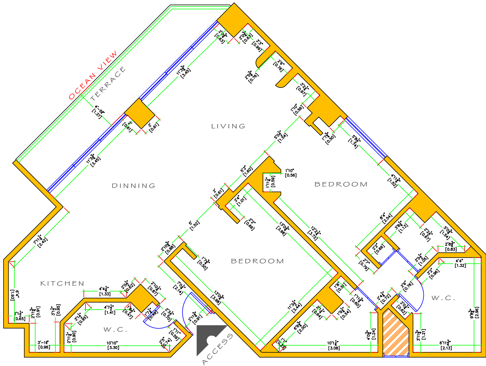
FLOOR PLAN
