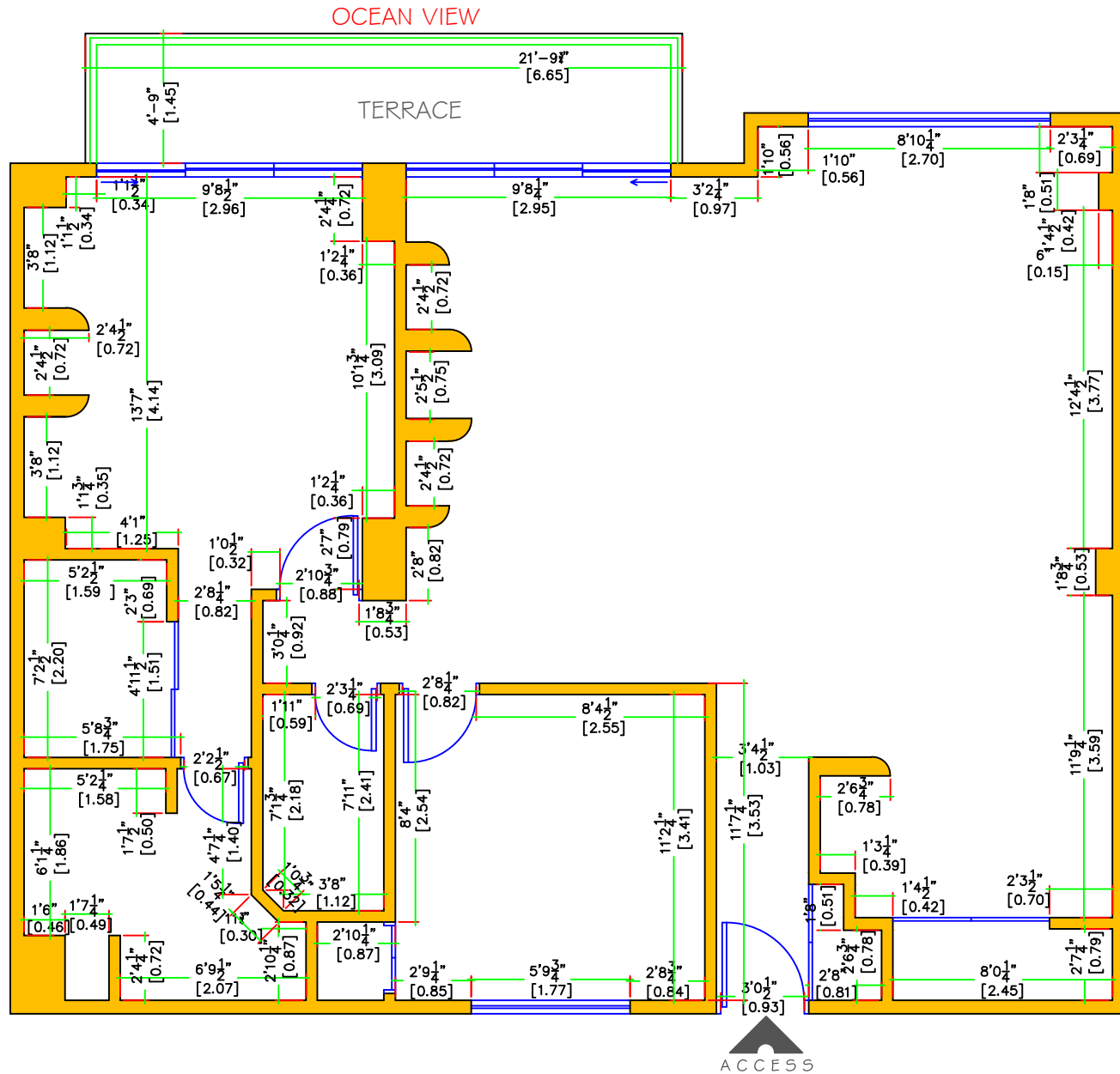
FLOOR PLAN
