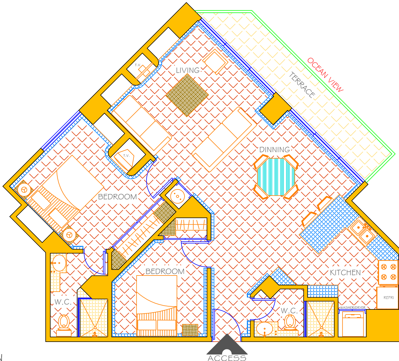
FLOOR PLAN
