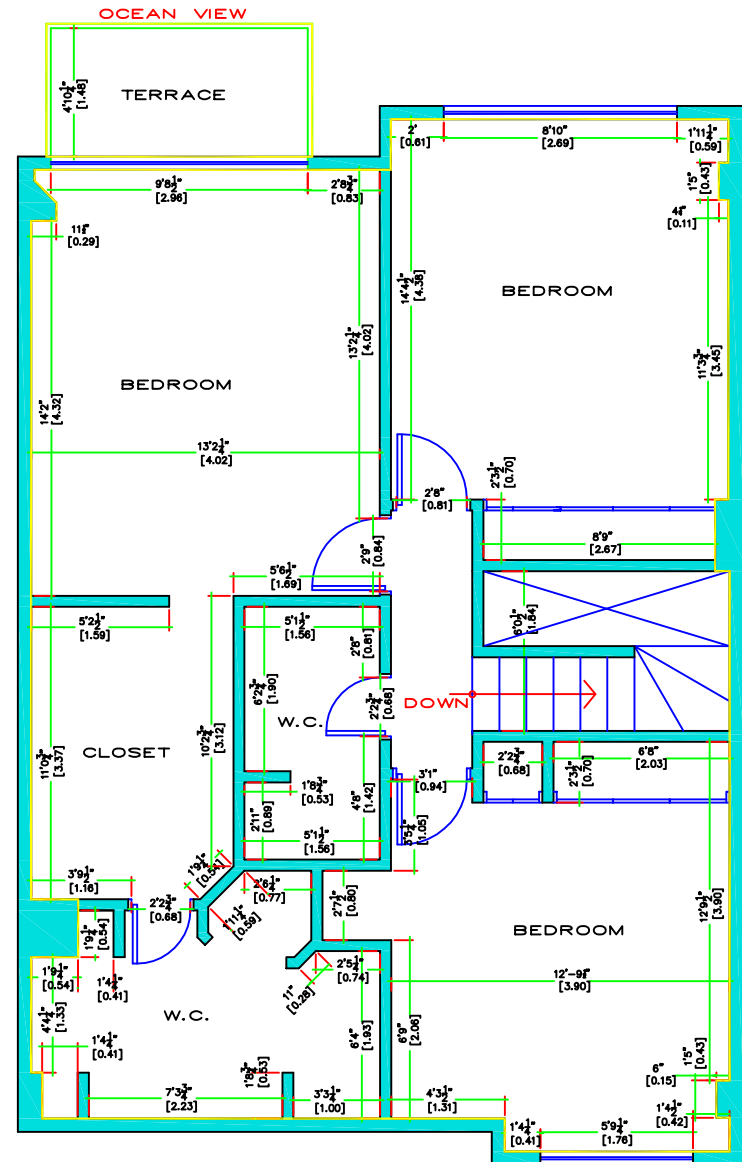
CM-902 SECOND FLOOR FLOOR PLAN
