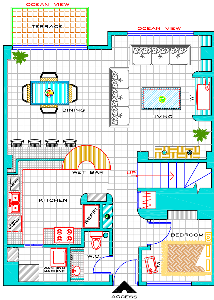
CM-902 FIRST FLOOR
