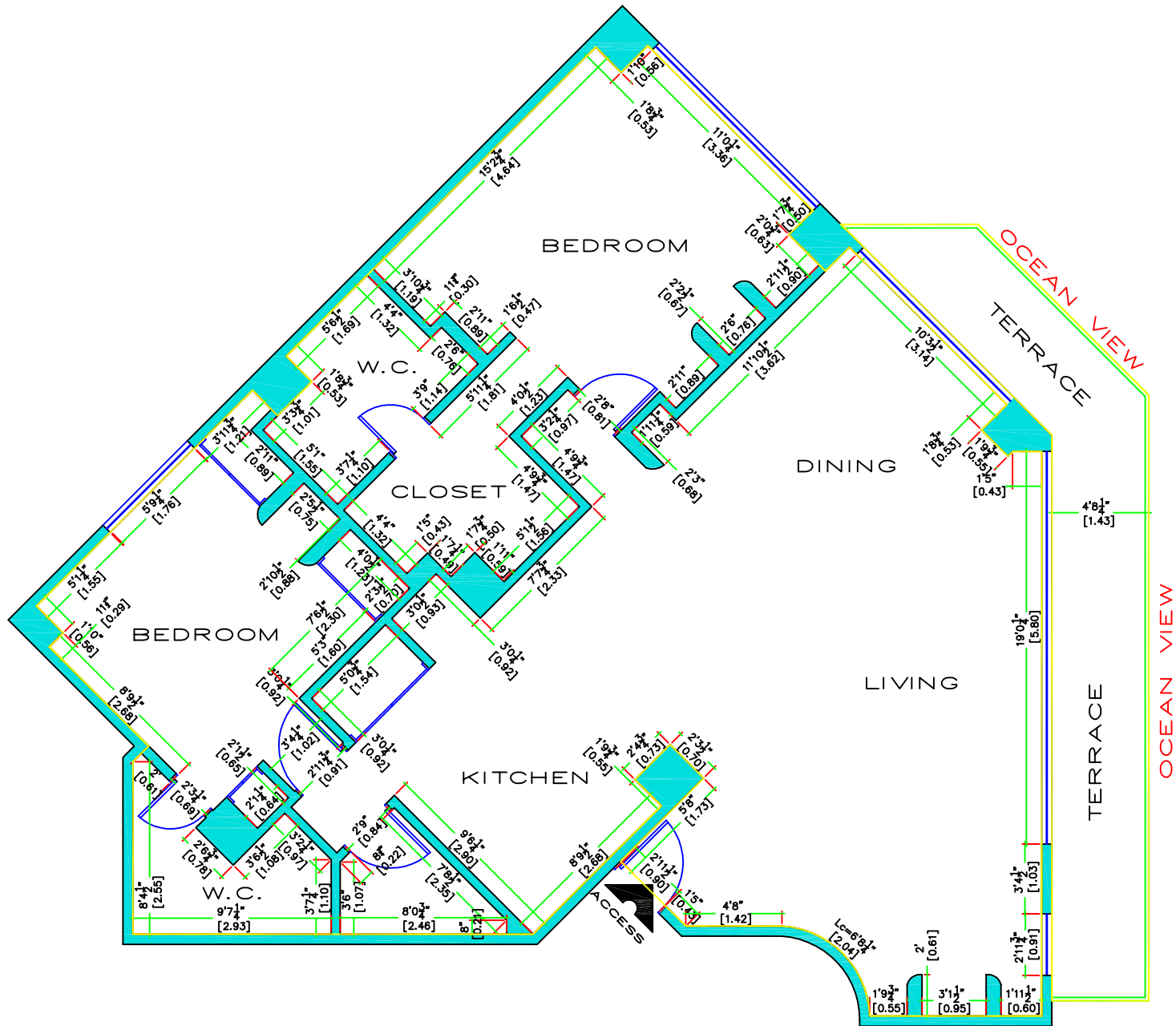
FLOOR PLAN
