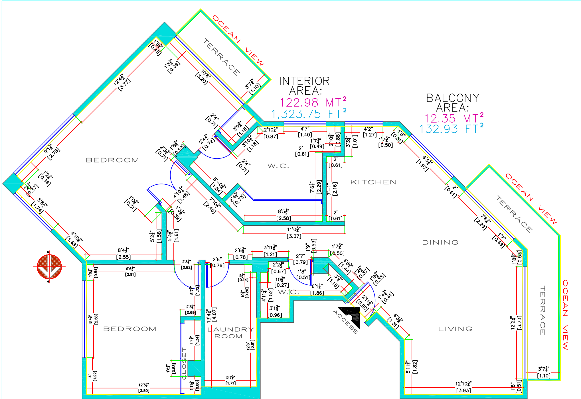
ARCHITECTURAL PLAN CM-901 MEASURE'S
